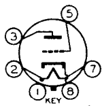
BOTTOM VIEW (G-6Q)
